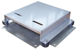
Base omega in acciaio inox con antivibranti "Omega" base made in stainless steel with anti-vibration mounts
