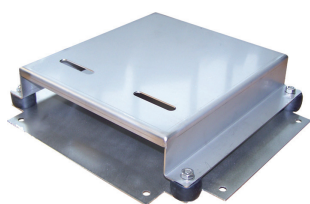
Base omega in acciaio inox con antivibranti "Omega" base made in stainless steel with anti-vibration mounts
